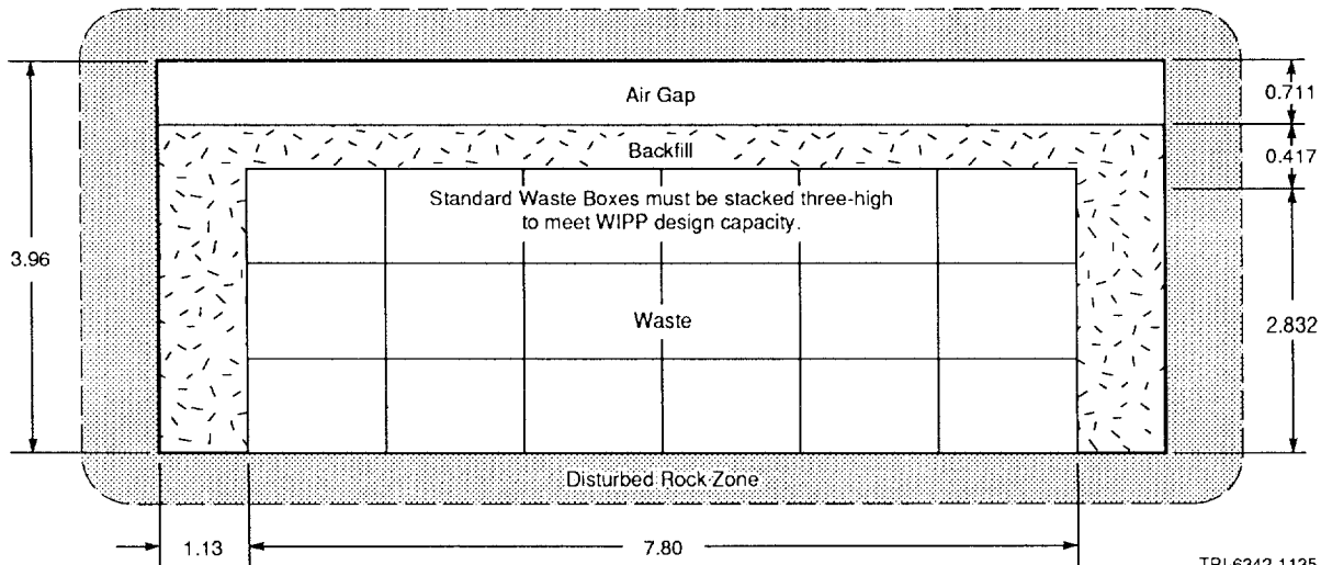
Figure 3.1-4. Ideal Packing of Standard Waste Boxes in Rooms and Drifts.
